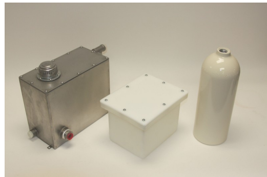
Stainless Steel and Polyethylene reservoirs.
